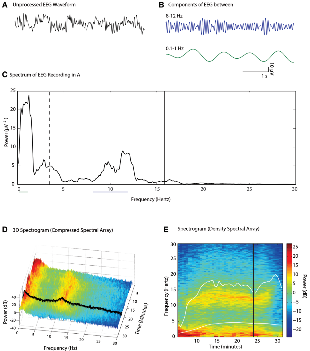
Fig. 3. Construction of the spectrogram. (A) A 10-s electroencephalogram (EEG) trace recorded under propofol-induced unconsciousness. (B) The electroencephalogram trace in A filtered into its two principal oscillations: the blue curve , an alpha (8 to 12 Hz) oscillation, and the green curve , a slow (0.1 to 1 Hz) oscillation. (C) The spectrum provides a decomposition of the electroencephalogram in A into power by frequency for all of the frequencies in a specified range. The range here is 0.1 to 30 Hz. Power at a given frequency is defined in decibels as the 10 times the log base 10 of the squared amplitude. The green horizontal line underscores the slow-delta frequency band and the blue horizontal line underscores the alpha frequency band used to compute the filtered signals in B. The median frequency, 3.4 Hz ( dashed vertical line ), is the frequency that divides the power in the spectrum in half. The spectral edge frequency, 15.9 Hz ( solid vertical line ), is the frequency such that 95% of the power in the spectrum lies below this value. (D) The three-dimensional (3D) spectrogram (compressed spectral array) displays the successive spectra computed on a 32-min electroencephalogram recording from a patient anesthetized with propofol.
