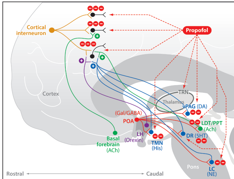
Fig. 4. Neurophysiological mechanisms of propofol's actions in the brain. Propofol enhances \gamma -aminobutyric acid receptor type A ( GABA_A )-mediated inhibition in the cortex, thalamus, and brainstem. Shown are three major sites of action: postsynaptic connections between inhibitory interneurons and excitatory pyramidal neurons in the cortex; the GABA_A ergic neurons in the thalamic reticular nucleus (TRN) of the thalamus; and postsynaptic connections between GABA_A ergic and galanergic (Gal) projections from the preoptic area (POA) of the hypothalamus and the monoaminergic nuclei, which are the tuberomammillary nucleus (TMN) that releases histamine (His), the locus ceruleus (LC) that releases norepinephrine (NE), the dorsal raphe (DR) that releases serotonin (5HT); the ventral periaqueductal gray (vPAG) that releases dopamine (DA); and the cholinergic nuclei that are the basal forebrain (BF), pedunculo-pontine tegmental (PPT) nucleus, and the lateral dorsal tegmental (LDT) nucleus that release acetylcholine (ACh). Also shown is the lateral hypothalamus (LH) that releases orexin. Adapted, with permission, from Brown, Purdon, and Van Dort: General anesthesia and altered states of arousal: A systems neuroscience analysis. Annu Rev Neurosci 2011; 34:601–28. Adaptations are themselves works protected by copyright. In order to publish this adaptation, authorization has been obtained both from the owner of the copyright of the original work and from the owner of copyright of the translation or adaptation.
